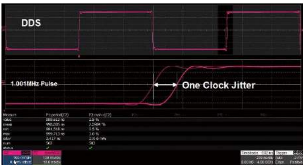
When a Square/Pulse waveform is generated by DDS, there will be a one-clock-jitter if the sampling rate is not an integer-related multiple of the output frequency. SDG2000X EasyPulse technology successfully overcomes this weakness in DDS designs and helps to produce low jitter Square/Pulse waveforms.
