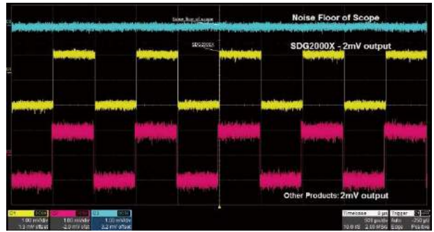
Low noise floor, improves signal-noise ratio.
