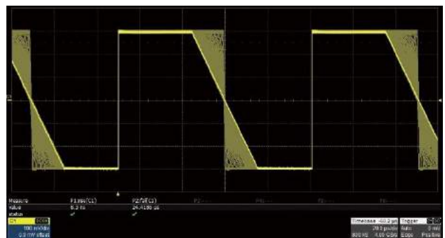
The rise/fall times can be set independently to the minimum of 8.4ns at any frequency and to the maximum of 22.4s. The adjustment step is as small as 100 ps.
